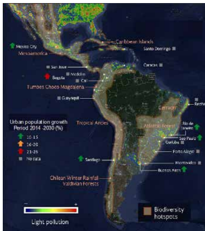
Figure 2.5.1: Light pollution, urban population growth and biodiversity hotspots in Latin America and the Caribbean.
