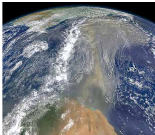
Saharan dust heading west towards South America and the Gulf of Mexico, 25 June 2015
